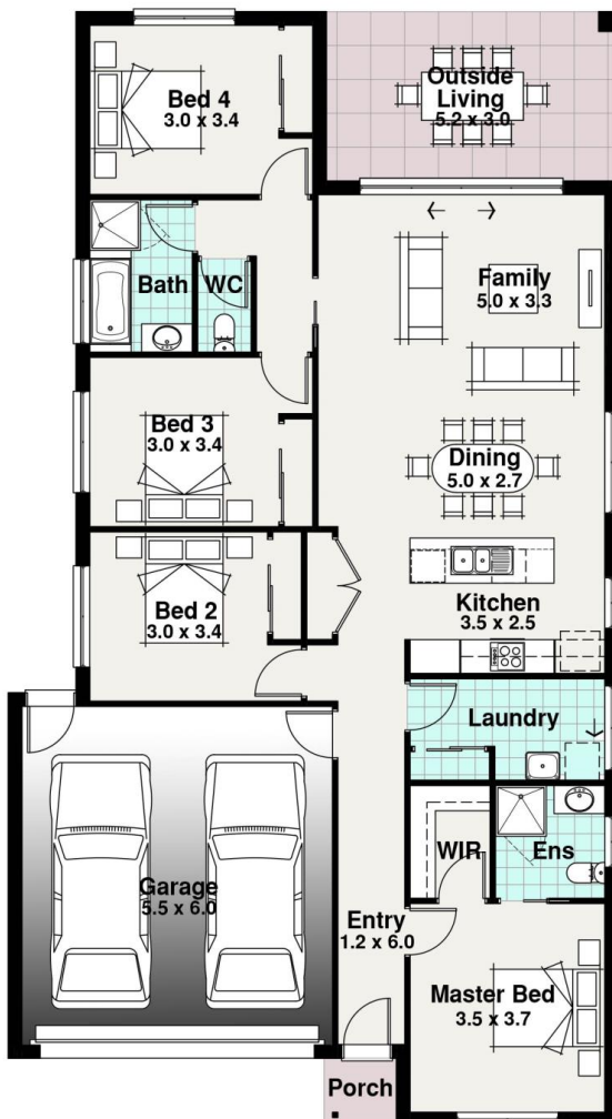
Floor plan shown is based on Traditional Facade.
